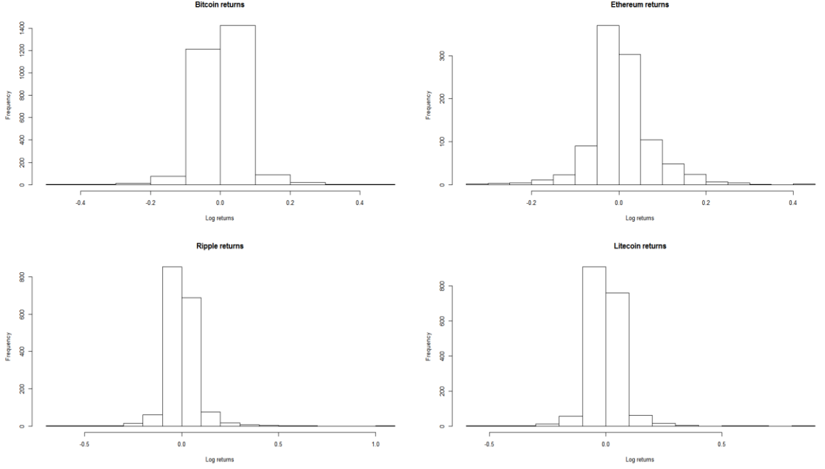
Figure 2 Histograms of log returns
