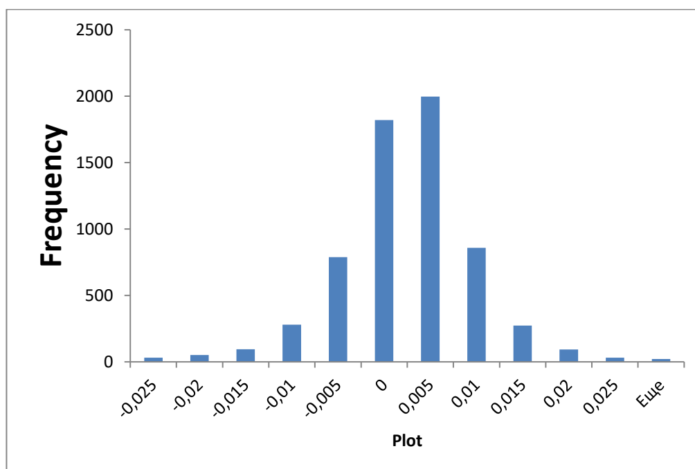
Figure A.7: Frequency distribution of GBPCHE, 1994-2019
