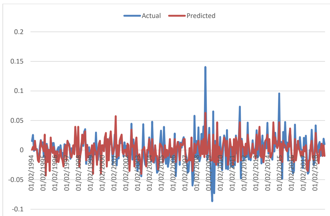
Figure H.4: Distribution of returns: actual vs estimated (from the regression model and the actual data): case of USDCAD
