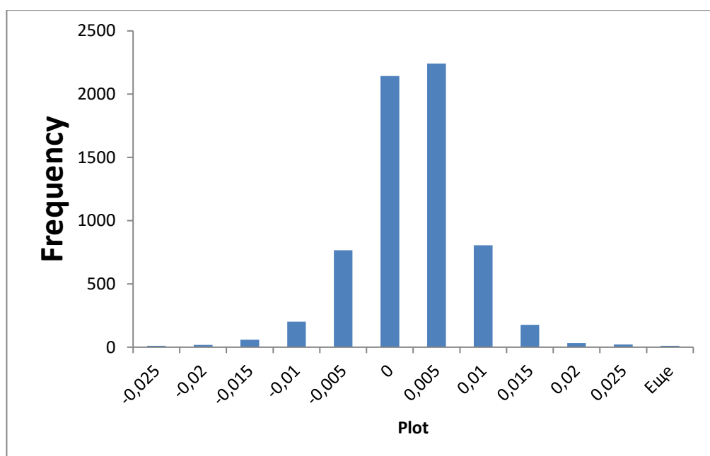
Figure A.7: Frequency distribution of GBPCHE, 1994-2019
