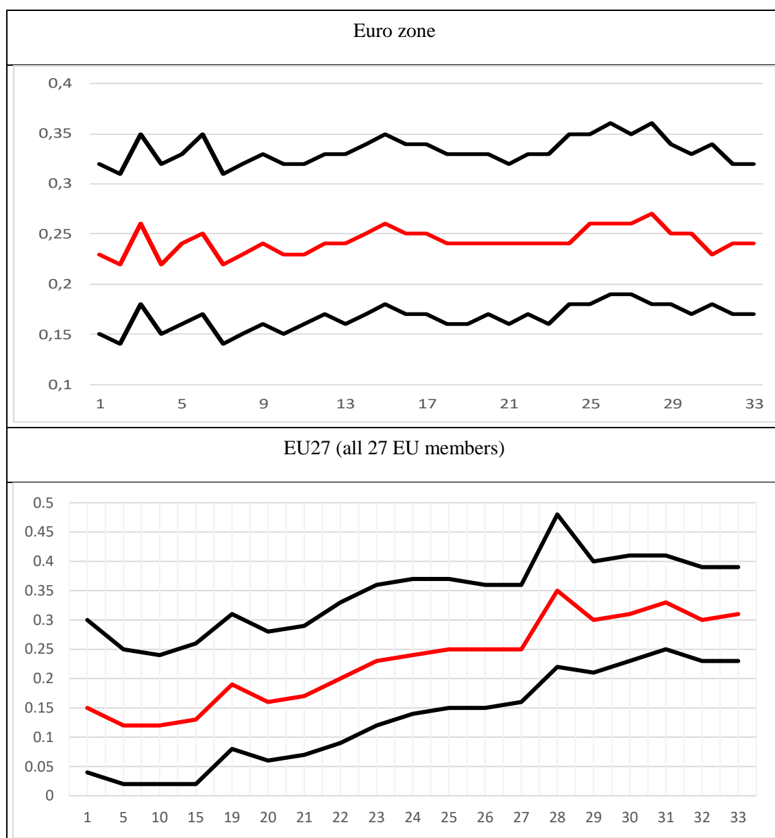
Figure 1: Recursive estimates of d as a measure of inflation persistence
