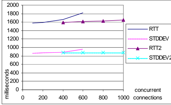
Fig. 11. R-GMA Consumer tests RTT and STDDEV are tests on single server RTT2 and STDDEV2 are distributed network tests
