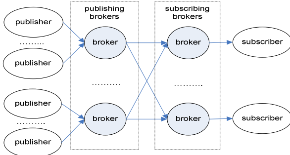
Fig. 5. Distributed architecture
