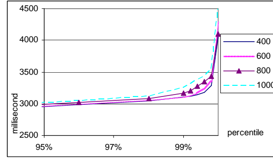
Fig. 14. R-GMA Consumer distributed network, percentile of RTT For a number of 400 ~ 1000 concurrent connections
