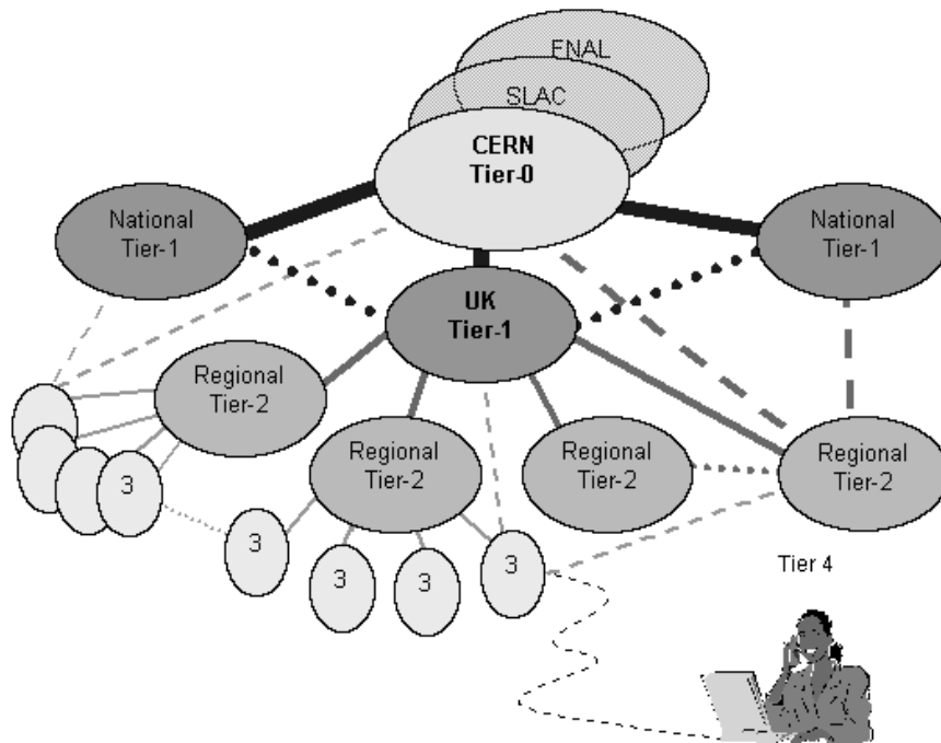
Figure 2 The tiered structure of the particle physics grid "GRIDPP" for the Large Hadron Collider experiments. The physical experiment CMS is located at the CERN Tier-
