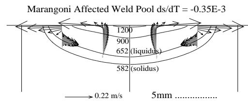
Figure 10a: Negative: Temperature and flow fields
